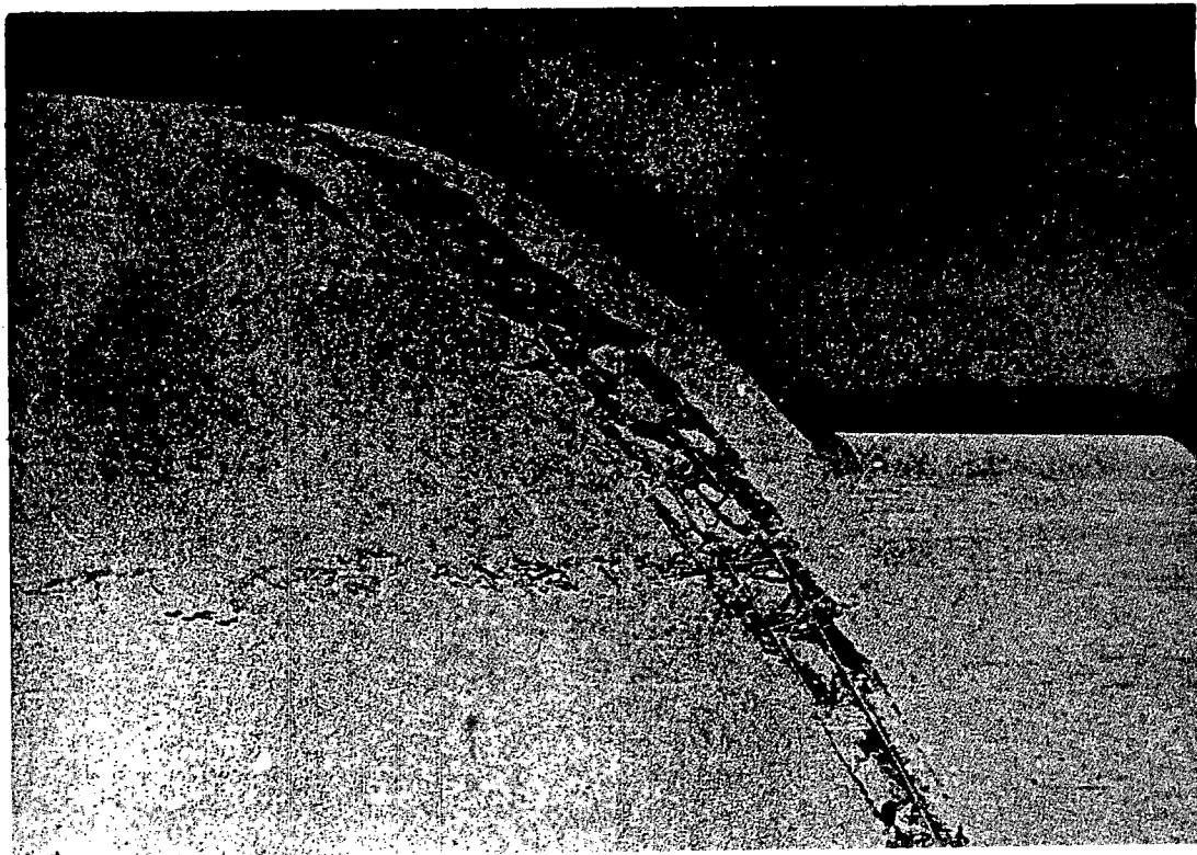
Fig. 12—Damage to side of concrete arch facing GZ at 70-psi overpressure region.
